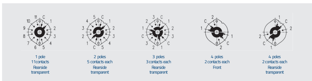
SM 30 · Contact surfaces as viewed from detent mechanism
