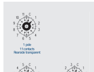
1 pole 11 contacts Rearside transparent
