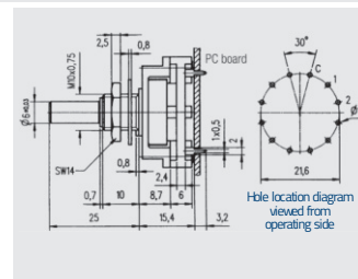
SM25 · Version for printed circuits
