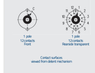
1 pole 12 contacts Front
