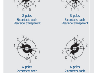
2 poles 5 contacts each Rearside transparent
