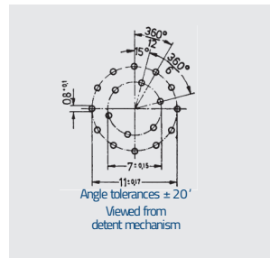
Contact arrangement for printed circuits
