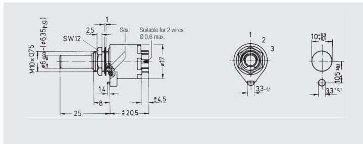
SB16 · MIL-version, shaft design A
