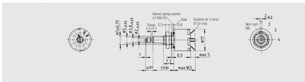
SB16 · Step switch with impulse contact
