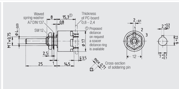
SB16 Standard version with soldering pins
