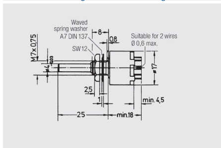
SB16 · Standard version with soldering lugs
