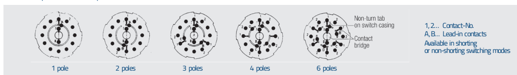
SB16 · Contact arrangements as viewed from detent mechanism
