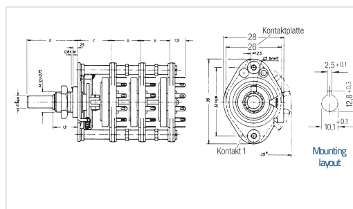
BS · Lever detent mechanism
