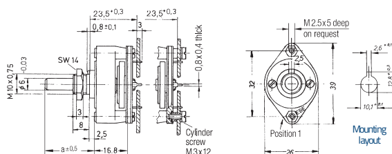
BS · PC board version
