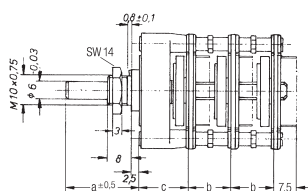
BS · Version with soldering lugs
